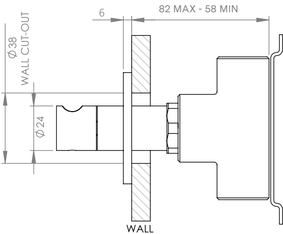
DIVERTER VIEW
