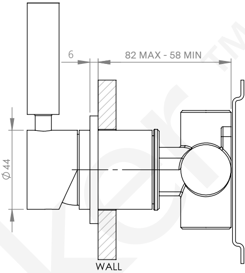
WALL MIXER VIEW
